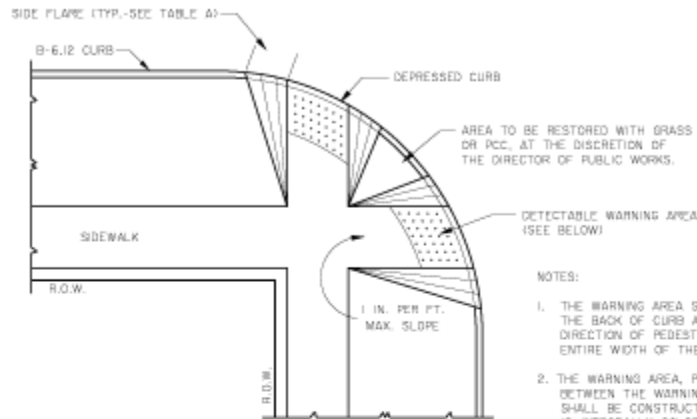
SIDEWALK RAMP PLAN
