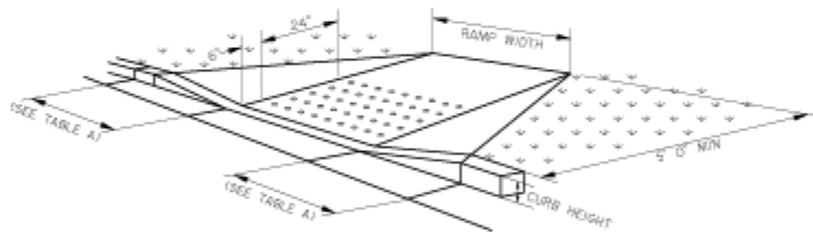
DETECTABLE WARNING DETAIL
