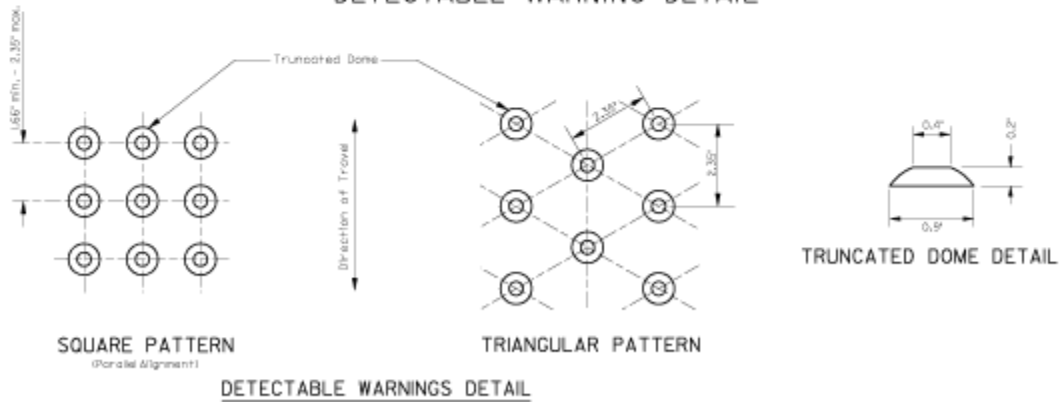
DETECTABLE WARNING DETAIL
