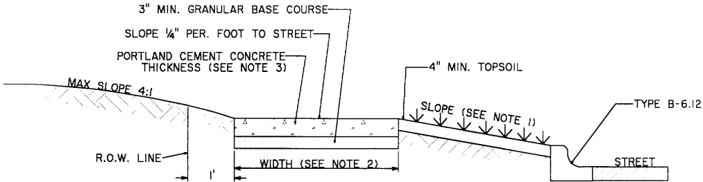
TYPICAL SIDEWALK SECTION IN CUT AREA
