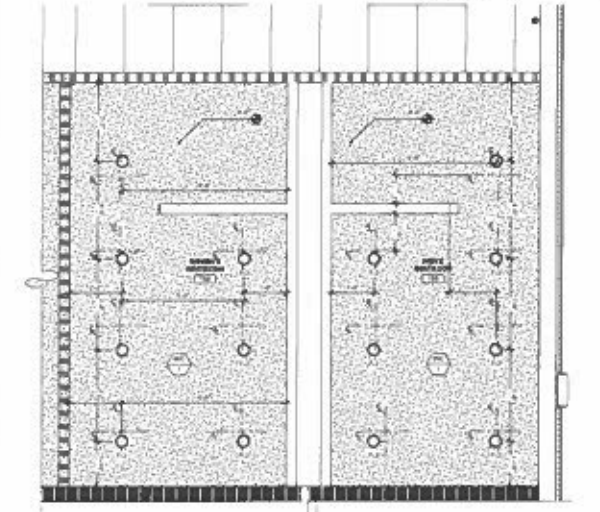
ENLARGED RESTROOM CEILING PLAN
