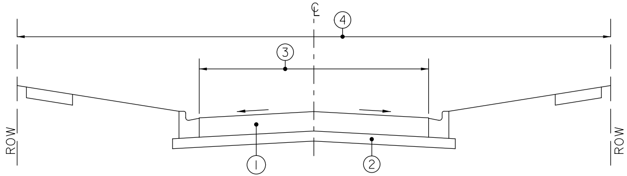
TYPICAL STREET CROSS SECTION - RIGID PAVEMENT
