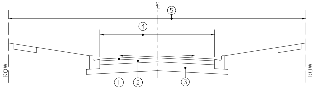
TYPICAL STREET CROSS SECTION - FLEXIBLE PAVEMENT
