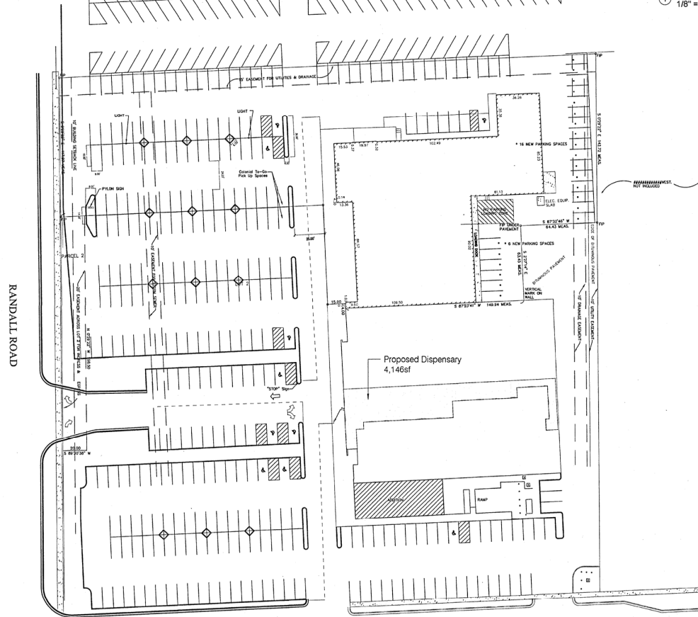
2 Site Plan 1" = 40'-0"
