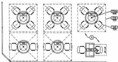
FURNITURE PLAN 1/4" = 1'-0"
