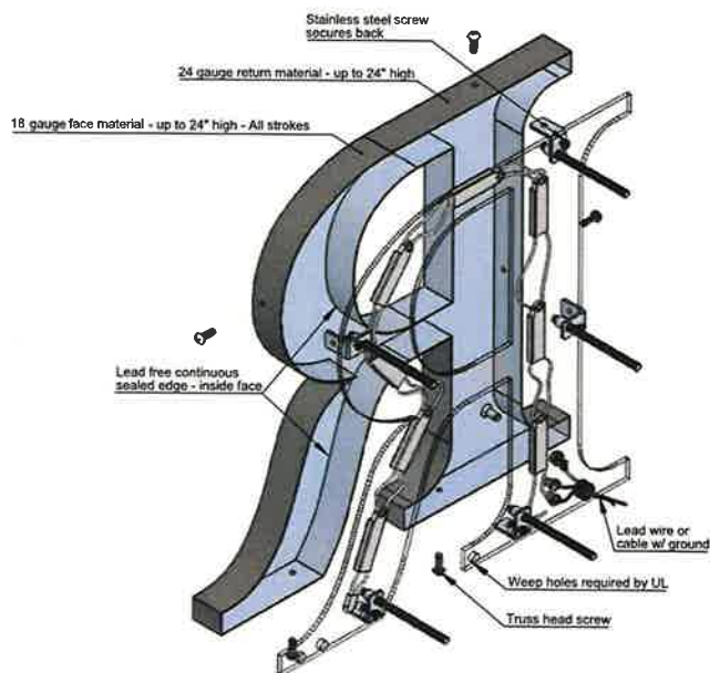
ISOMETRIC BACK VIEW
