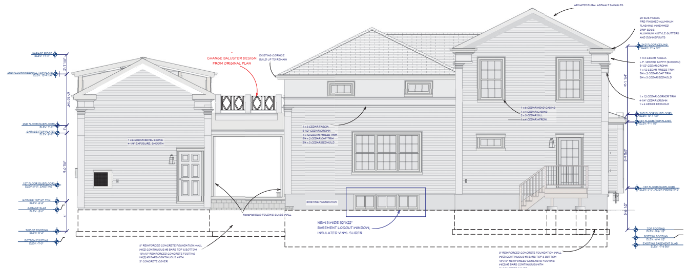
REAR ELEVATION
