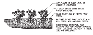
4 ANNUAL, PERENNIAL, & GROUNDCOVER DETAIL Not To Scale 329361-03
